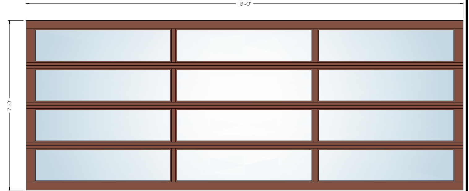
18' X 7' 3-LITE
