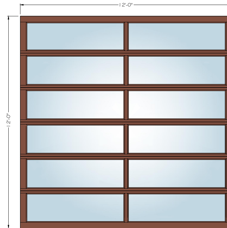
12' X 12' (2 / 3 / 4 - OPTIONALS LITES)
