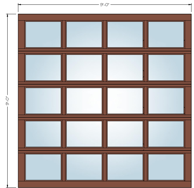
9' X 9' 4 - LITE
