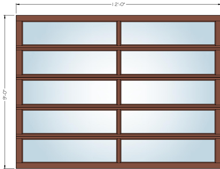
12' X 9' (2 / 3 / 4 - OPTIONALS LITES)
