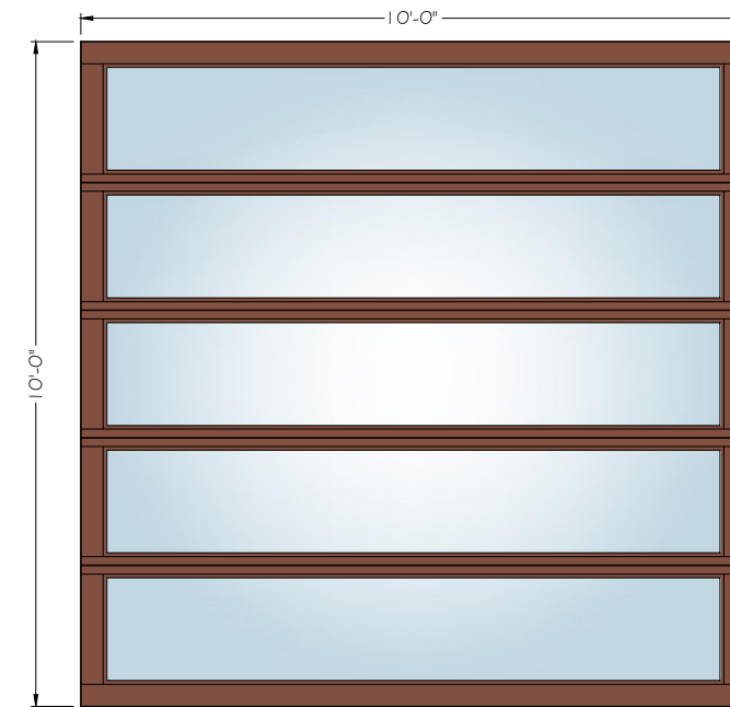
10' X 10' FULL LITE
