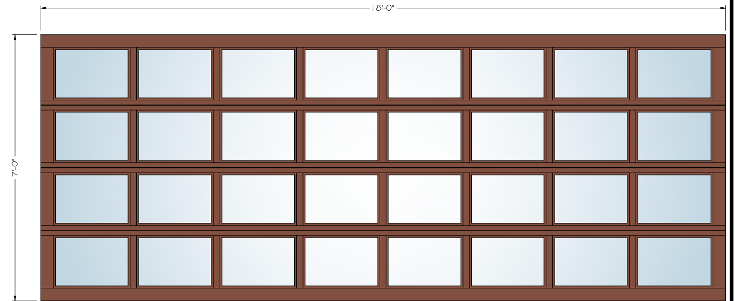
18' X 7' 8-LITE
