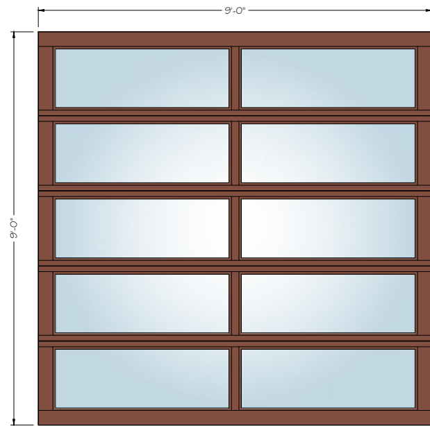
9' X 9' 2 - LITE
