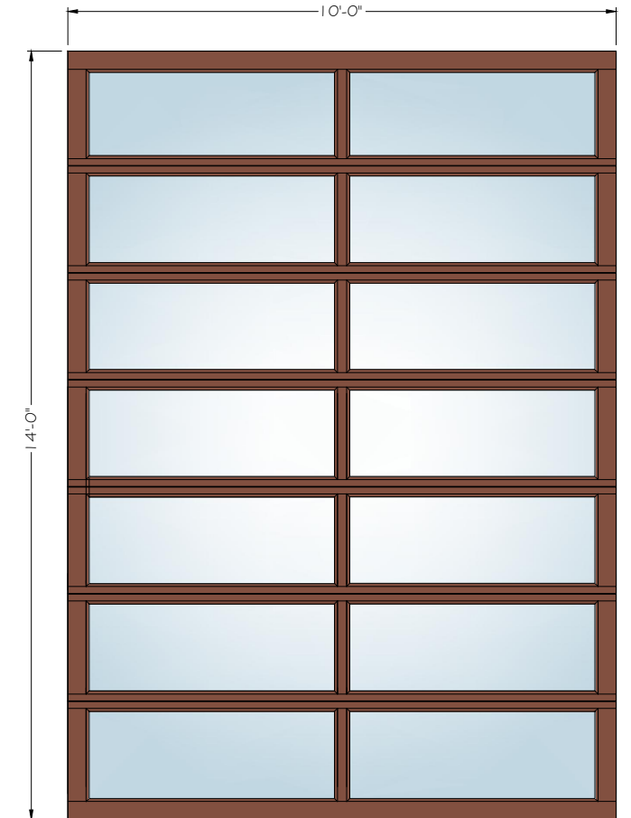
10' X 14' (2 / 3 / 4 - OPTIONALS LITES)
