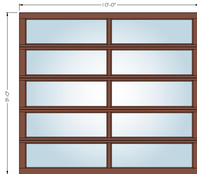
10' X 9' (2 / 3 / 4 - OPTIONALS LITES)
