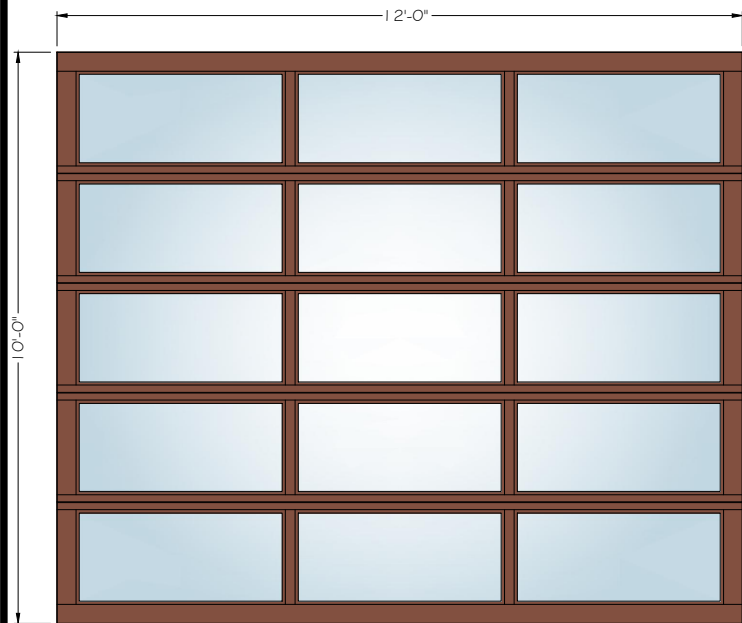
12' X 10' 3 - LITE
