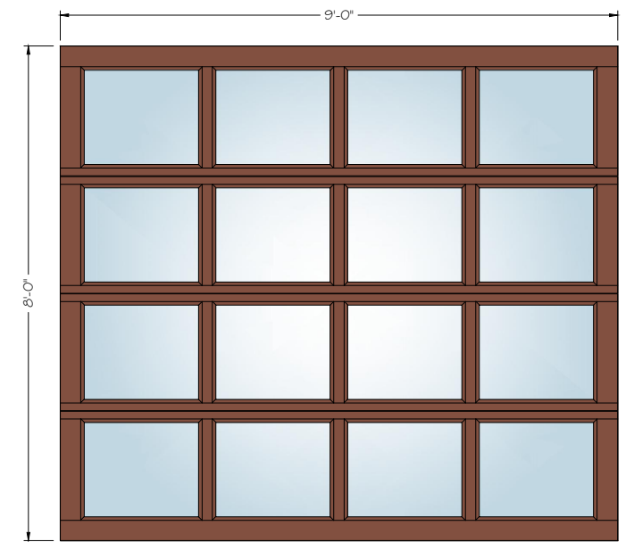
9' X 8' 4 - LITE
