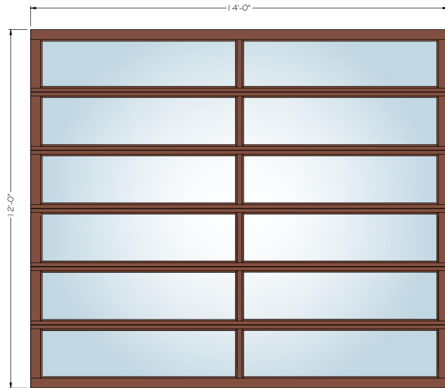
14' X 12' ( 3 / 4 - OPTIONALS LITES)
