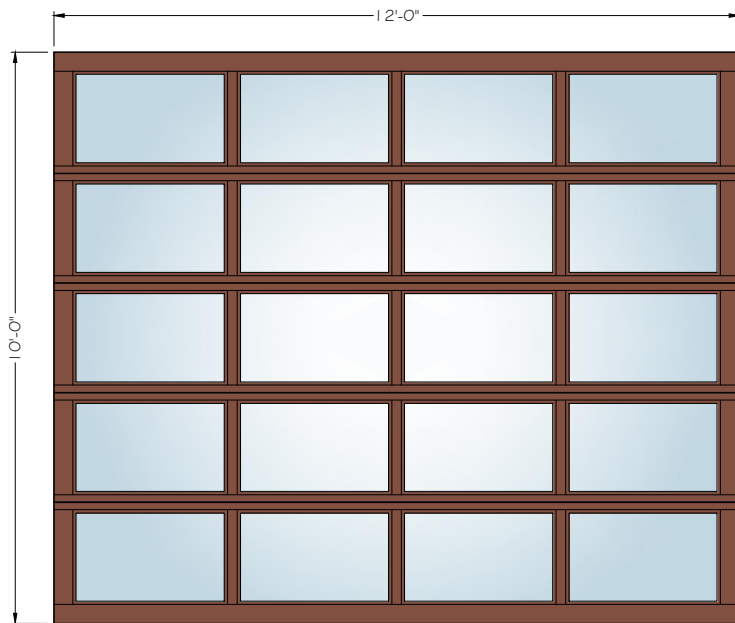
12' X 10' 4 - LITE
