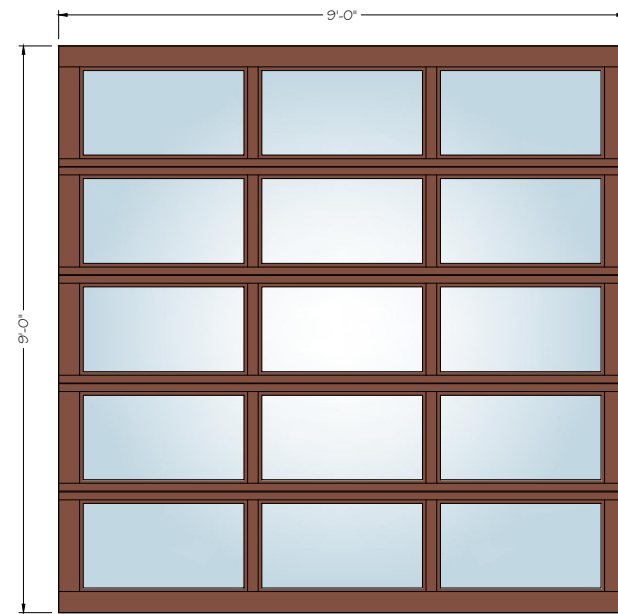
9' X 9' 3 - LITE
