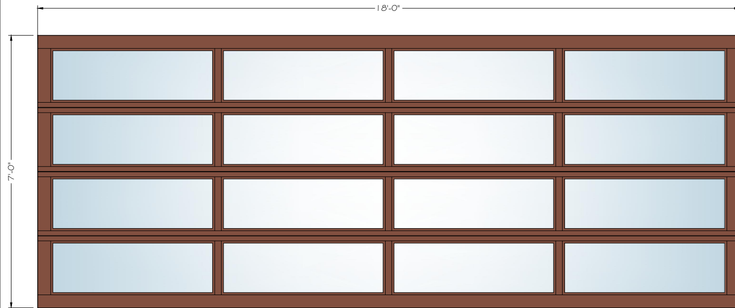
18' X 7' 4-LITE
