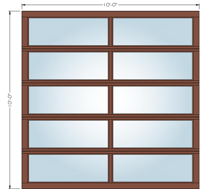
10' X 10' 2 - LITE
