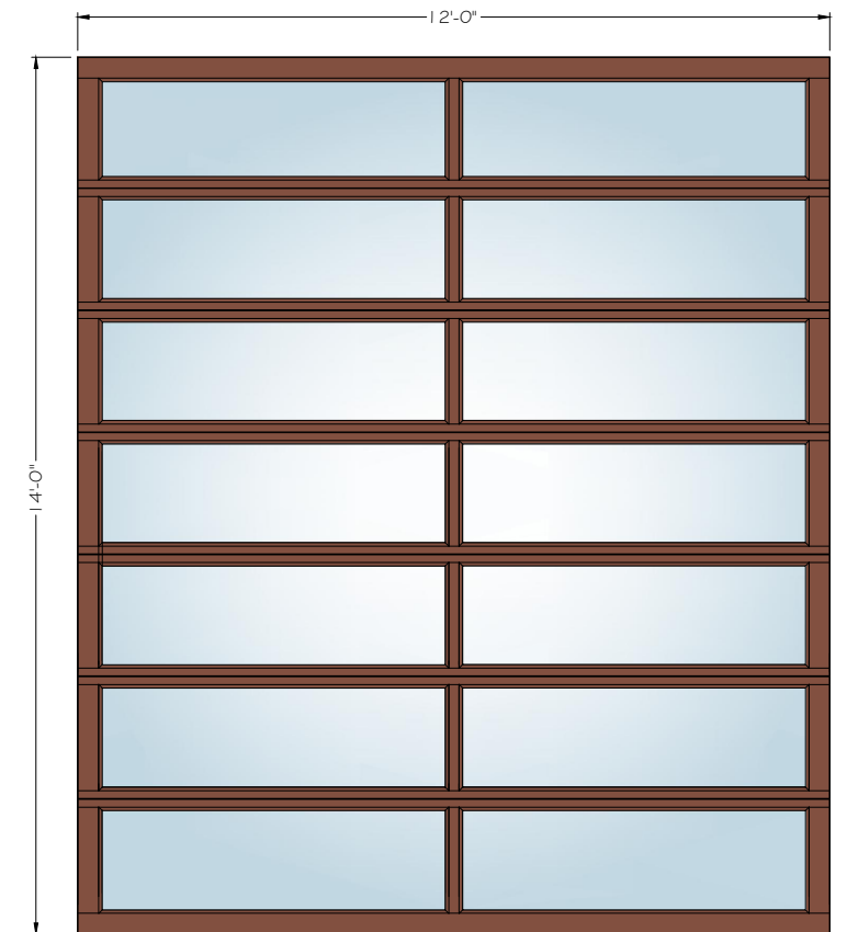
12' X 14' (2 / 3 / 4 - OPTIONALS LITES)
