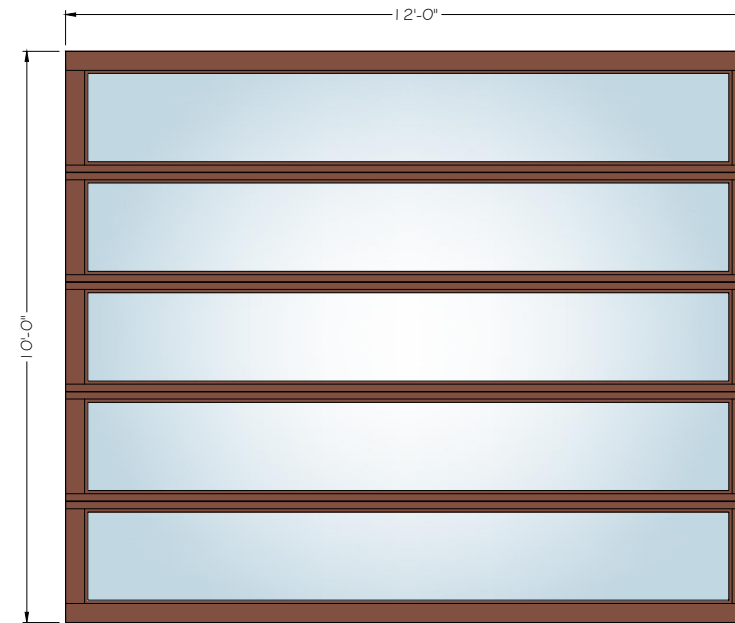
12' X 10' FULL LITE
